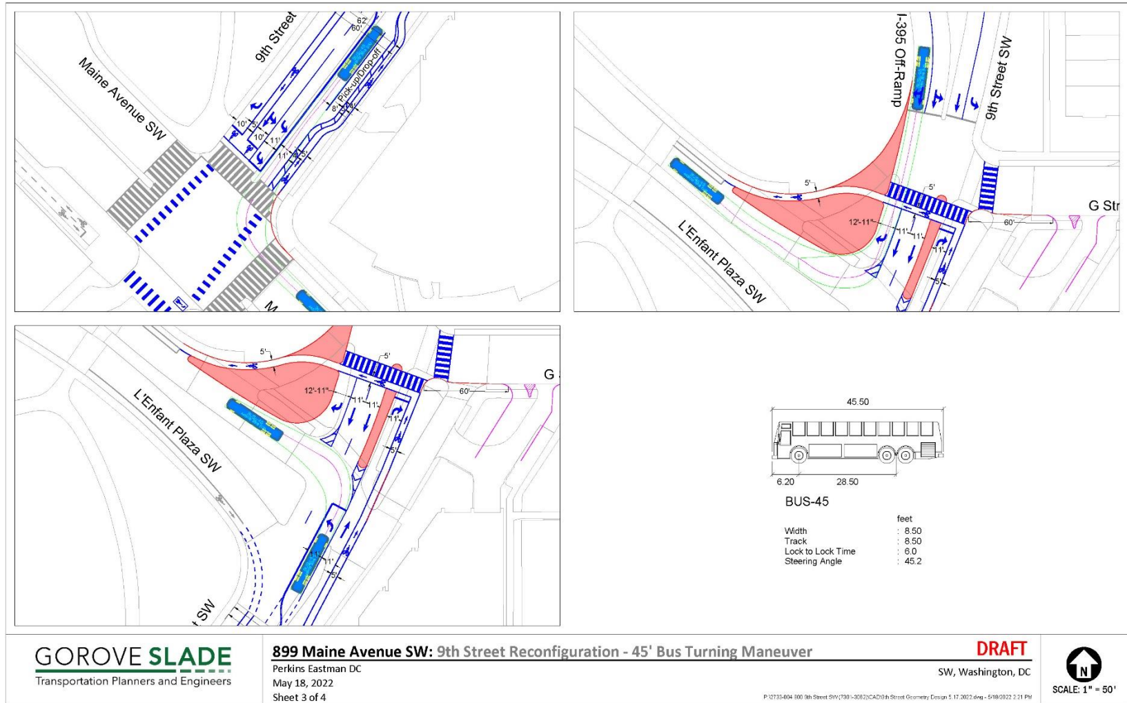
Figure 3: 45' Bus Turning Maneuvers
