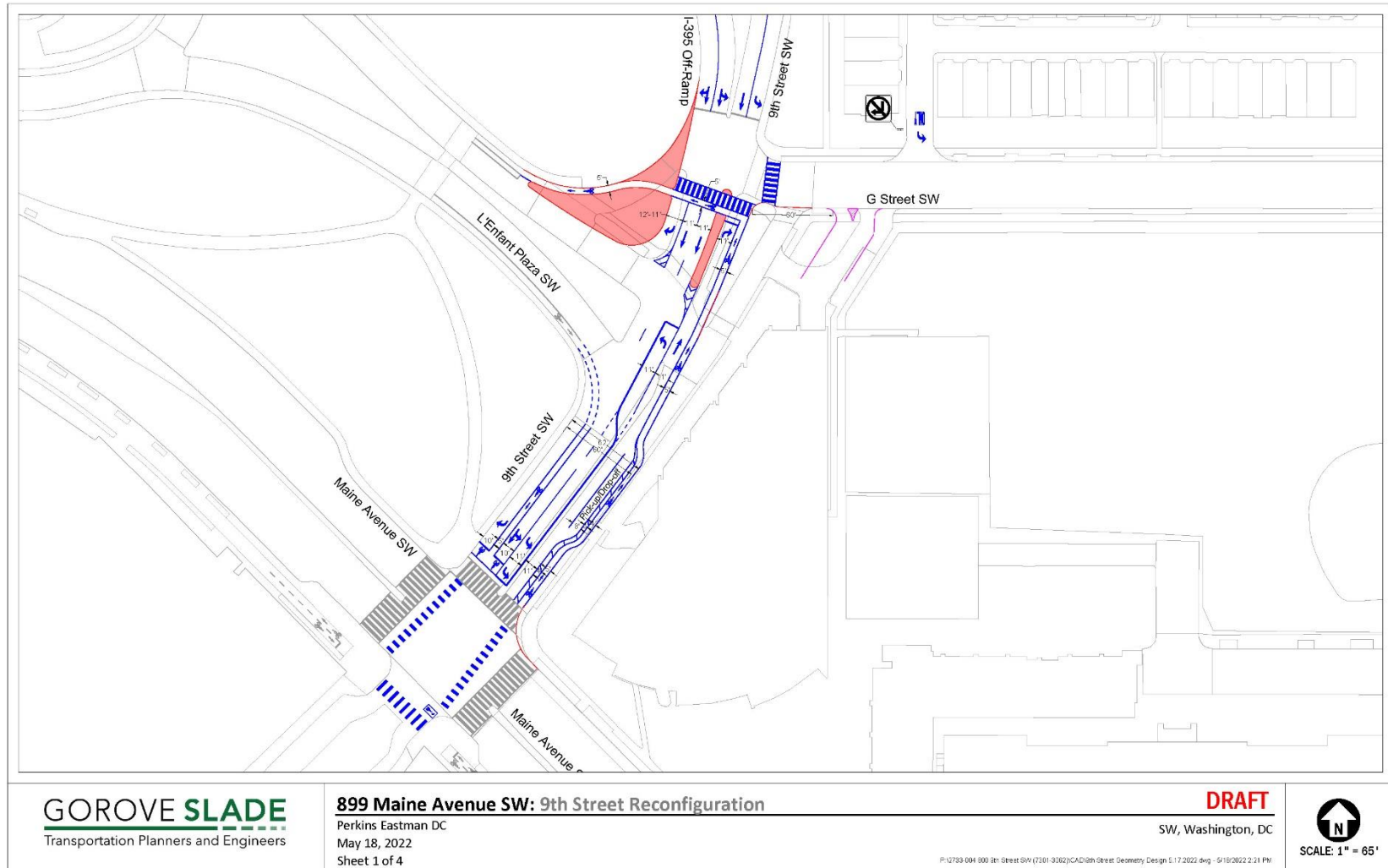
Figure 1: 9 th & G Street Reconfiguration
