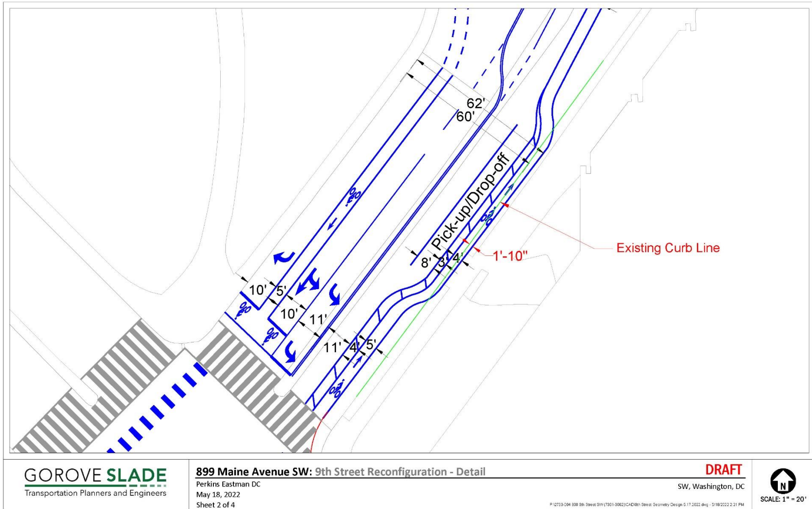
Figure 2: 9th Street Reconfiguration
